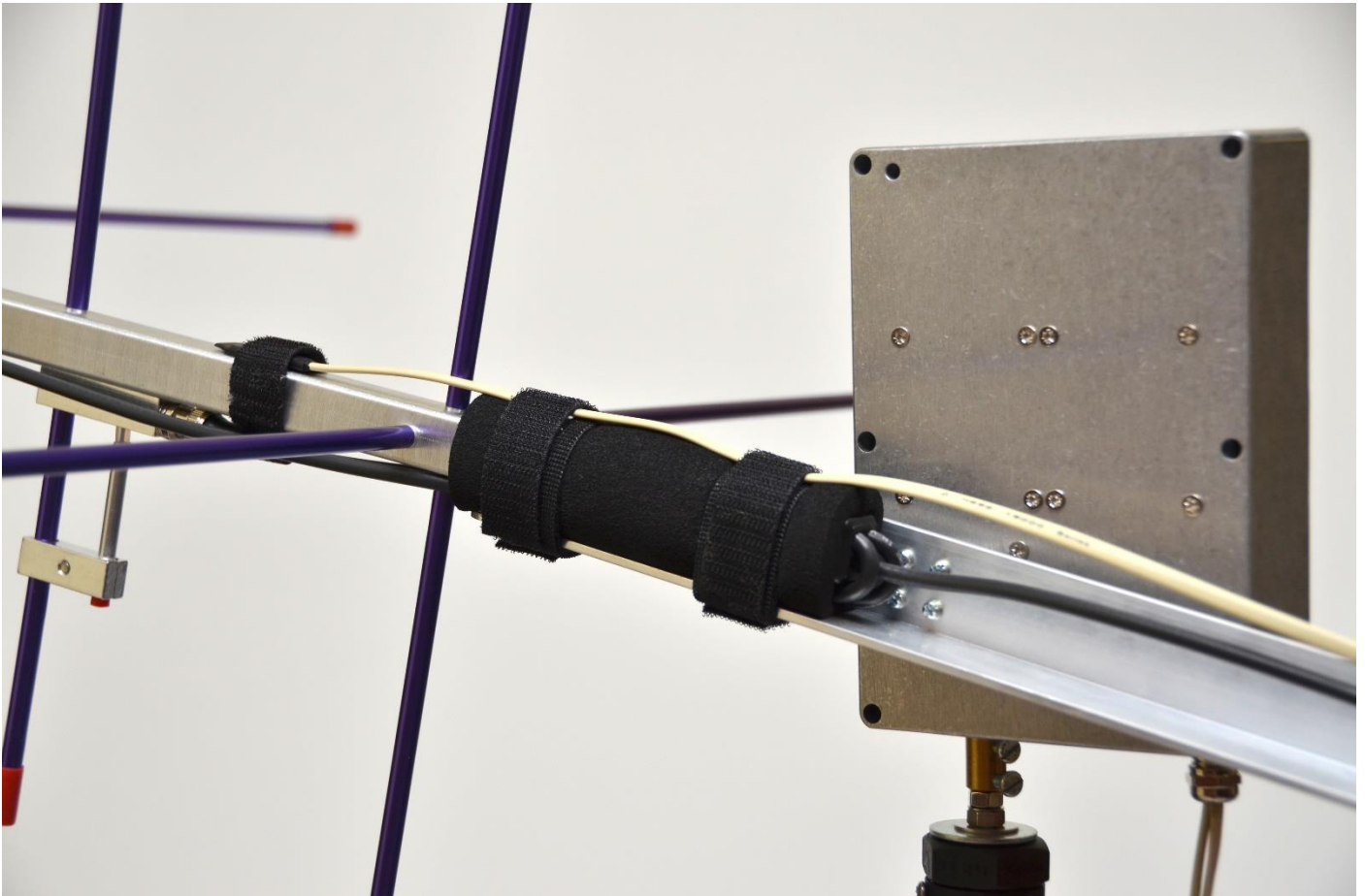
Figure 5 – Antenna and Lift Arm
