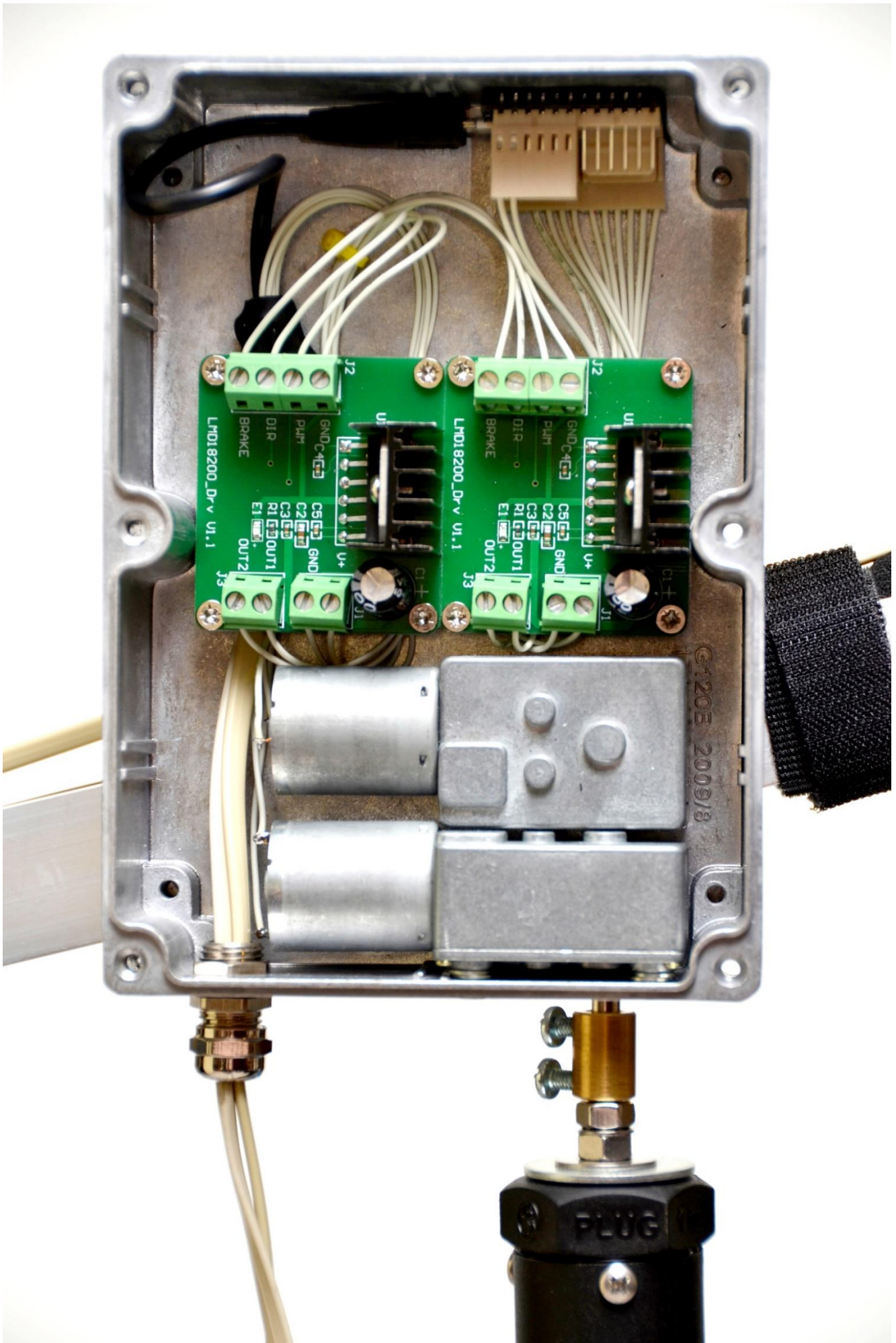
Figure 6 – Construction Details
