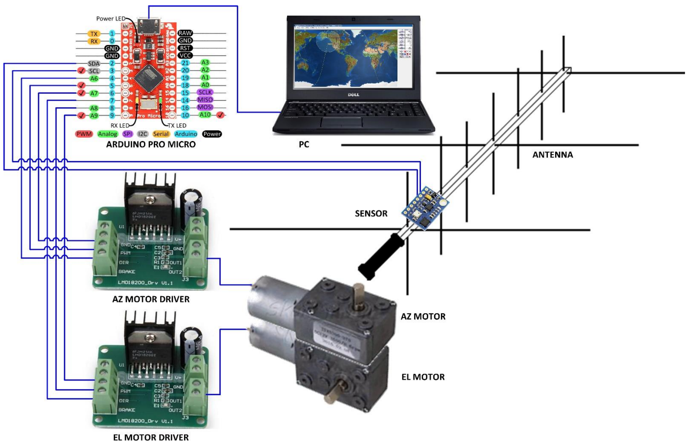
Figure 4 - Pictorial Schematic Diagram
